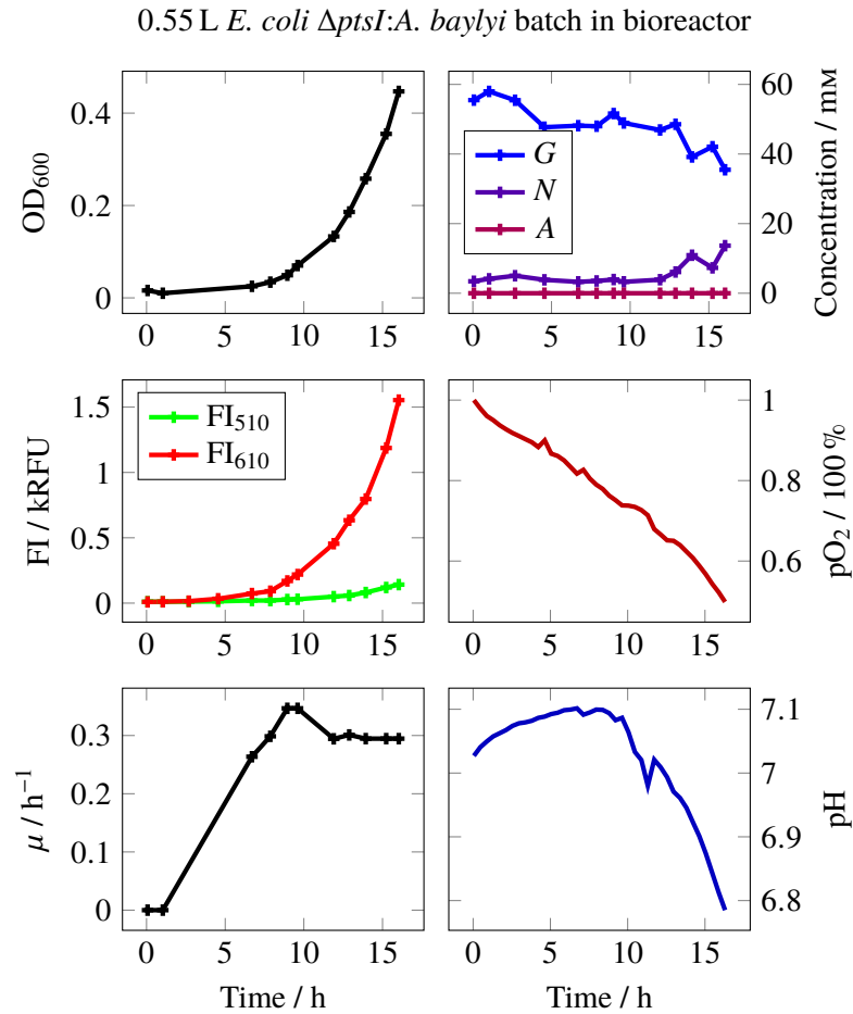
Figure 4.4 E. coli \Delta ptsI:A. baylyi -batch had the longest lag phase of this work, 5 h. Unfortunately the OD_{600} measurements were mostly unsuccessful during the first 5 h, and consequently the specific growth rates during that interval could not be estimated. Like in AB cultivation, pH rose from the initial value. G stands for glucose, N for gluconate, and A for acetate. FI_{510} denotes fluorescence intensity corresponding to sfGFP wavelengths and FI_{610} corresponds to mScarlet.
