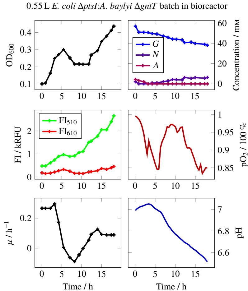
Figure 4.6 EC \Delta ptsI:AB\Delta gntT -batch was the most notable of the six cultures, because neither EC \Delta ptsI nor AB \Delta gntT could grow by themselves. The pO_2 signal correlated well with the observed growth in OD_{600} . G stands for glucose, N for gluconate, and A for acetate. FI_{510} denotes fluorescence intensity corresponding to sfGFP wavelengths and FI_{610} corresponds to mScarlet.
