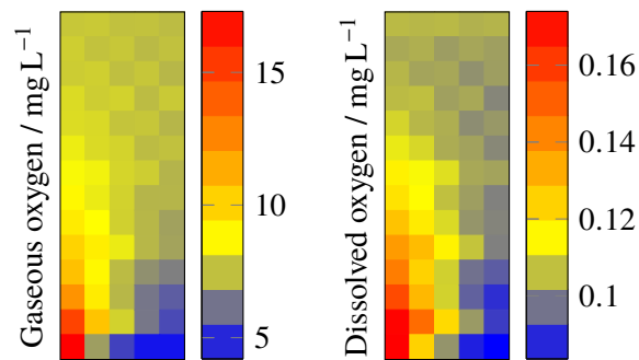
Figure 4.8 Distribution of oxygen in the large reactor at 10 h during batch cultivation of E. coli . Clearly the oxygen transfer was limiting throughout the reactor, but even then the extent of limitation was heterogeneously distributed. An oxygen-deprived zone is found at bottom of the reactor next to the wall. Surface aeration is slightly visible at top of the reactor, but it's contribution to overall aeration is negligible.
