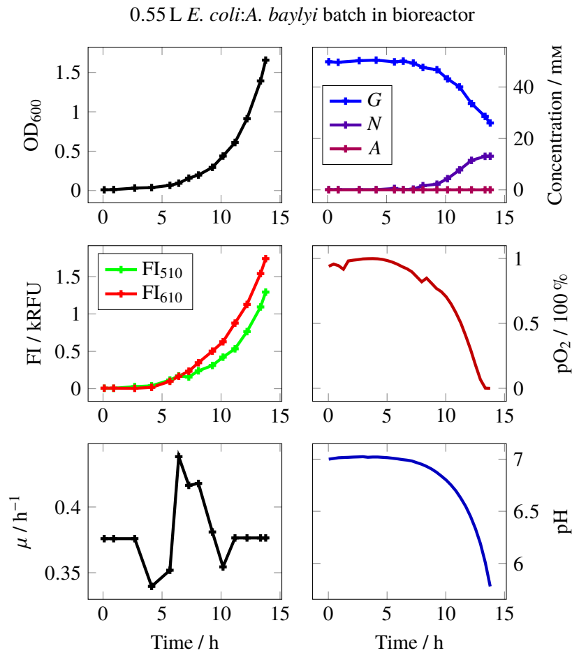
Figure 4.3 EC:AB-batch had consistently highest specific growth rates in this work. It also achieved the highest glucose conversion of almost 50 % within 14h. G stands for glucose, N for gluconate, and A for acetate. FI 510 denotes fluorescence intensity corresponding to sfGFP wavelengths and FI 610 corresponds to mScarlet.
