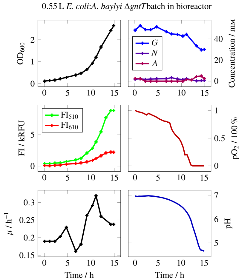
Figure 4.5 EC : AB \Delta gntT -batch reached the highest OD_{600} of this work, 2.64. The growth of both FI_{510} and FI_{610} signals indicate that both EC and AB \Delta gntT have grown in the co-culture. Also the quick consumption of initial acetate and the late reoccurrence of it imply that AB \Delta gntT has been active in the culture, consuming acetate excreted by EC . Oxygen limitation and possibly also low pH seem to have affected the culture towards the end of cultivation. G stands for glucose, N for gluconate, and A for acetate. FI_{510} denotes fluorescence intensity corresponding to sfGFP wavelengths and FI_{610} corresponds to mScarlet .
