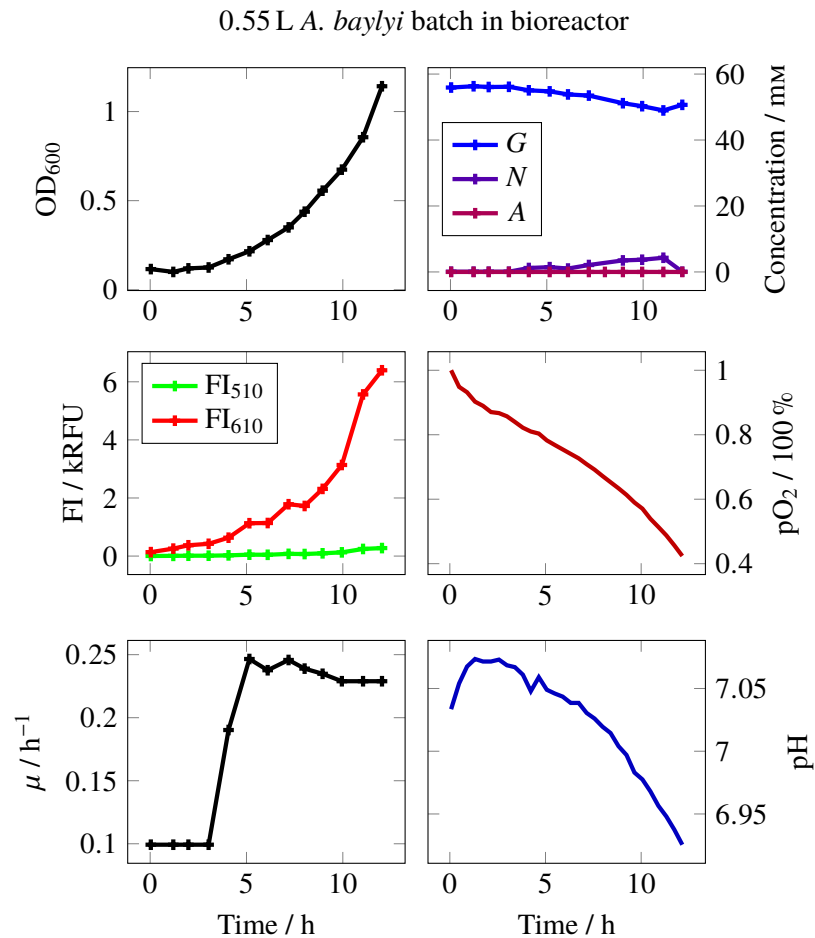
Figure 4.2 AB-batch reached an OD_{600} higher than EC, but the amount of glucose converted is much lower. Likewise the change in culture pH was very small. It seems therefore that A. baylyi cells have a higher optical density than E. coli . On the other hand, oxygen tension decreased well below the minimum found in EC culture, which indicates that the obligatorily aerobic A. baylyi consumed oxygen at a higher rate than E. coli , provided the aeration in both cultures was equal. G stands for glucose, N for gluconate, and A for acetate. FI_{510} denotes fluorescence intensity corresponding to sfGFP wavelengths and FI_{610} corresponds to mScarlet .
