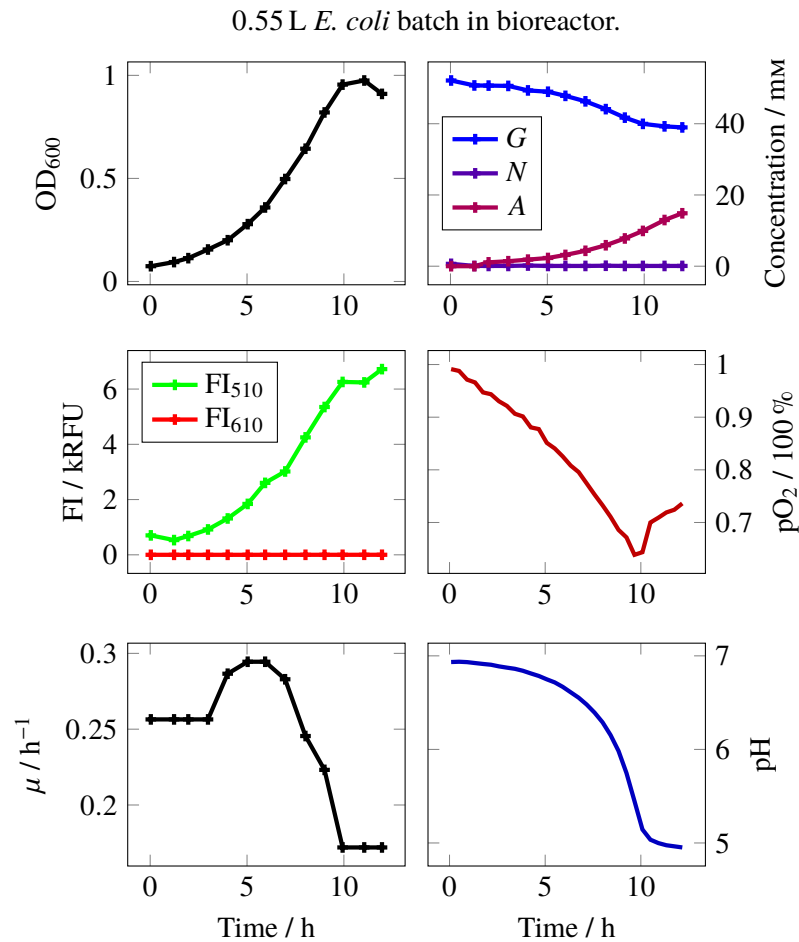
Figure 4.1 EC-batch displayed a typical batch growth curve: exponential growth until the accumulated acetate and medium pH became inhibitory. It is noted that the sharp inverse peak of pO 2 signal corresponds very accurately to the observed cease of growth. Another point worth noticing is that EC could achieve only about a 20% conversion of glucose substrate before the conditions became inhibitory. If the cultivation were continued over the 12 h, the calculated specific growth rate (lower left corner) would have fallen to 0 and possibly below at the end. G stands for glucose, N for gluconate, and A for acetate. FI 510 denotes fluorescence intensity corresponding to sfGFP wavelengths and FI 610 corresponds to mScarlet.
