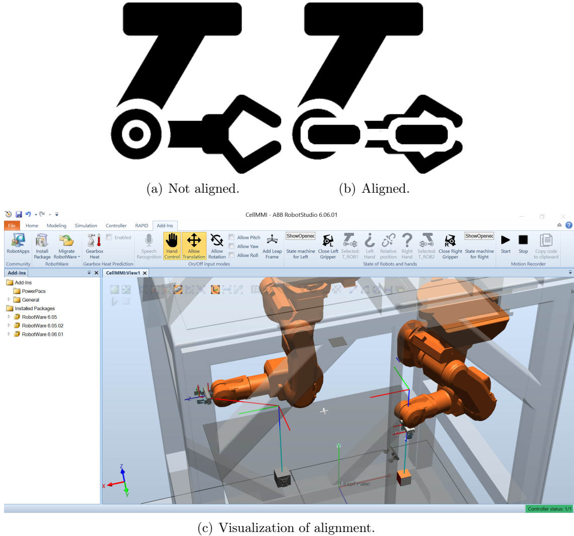
Figure 4.15 Alignment state feedback. The icon will change whenever the target frames are aligned to a piece. A dark cyan line is added to the aligned piece.
