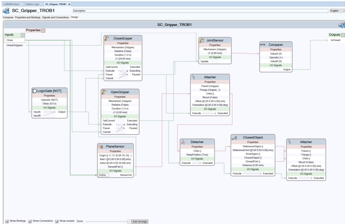
Figure 4.7 Gripper smart components design. Connections between the components and their properties define the behaviour of the gripper with the rest of the station.
