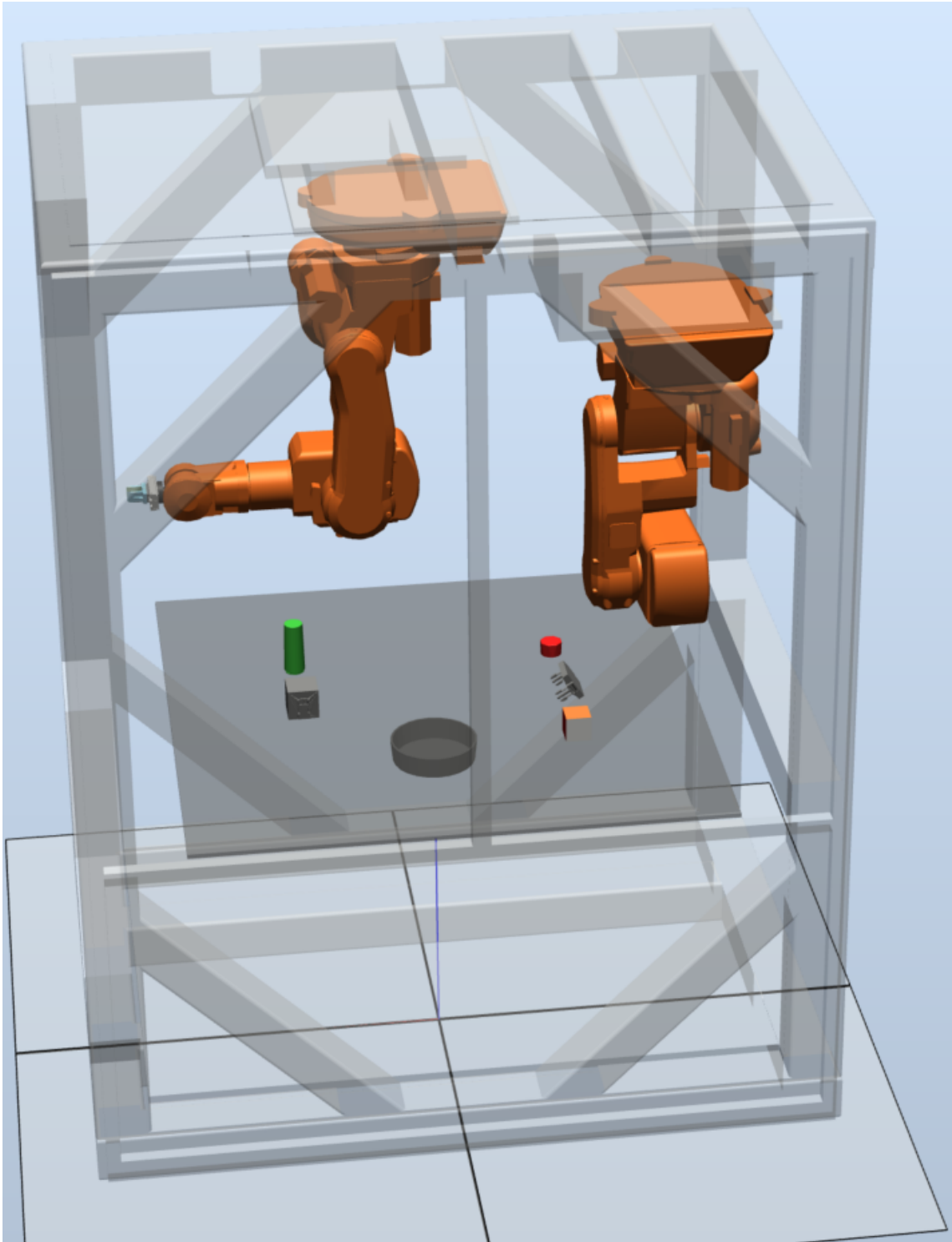
Figure 3.6 Testing environment used for making the programs using the interface.
