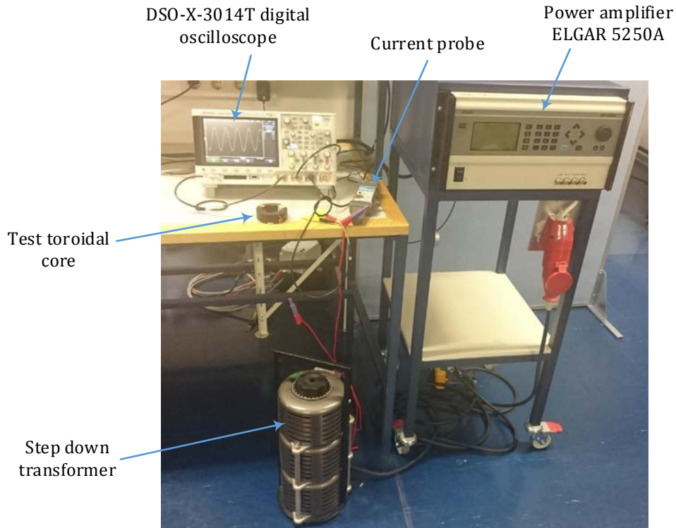
Figure 6.2: Laboratory setup.
