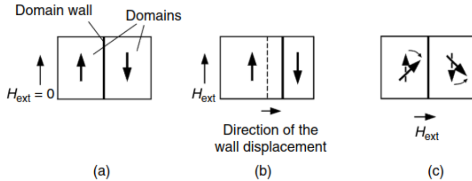
Figure 3.4: Magnetization of a ferromagnetic sample: (a) no applied external field; (b) with applied (c) rotation of the domain magnetic moments under applied external field H_{\text{ext}} [3].
