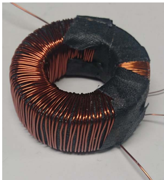
Figure 5.3: The prototype of 2605SA1 amorphous core.
