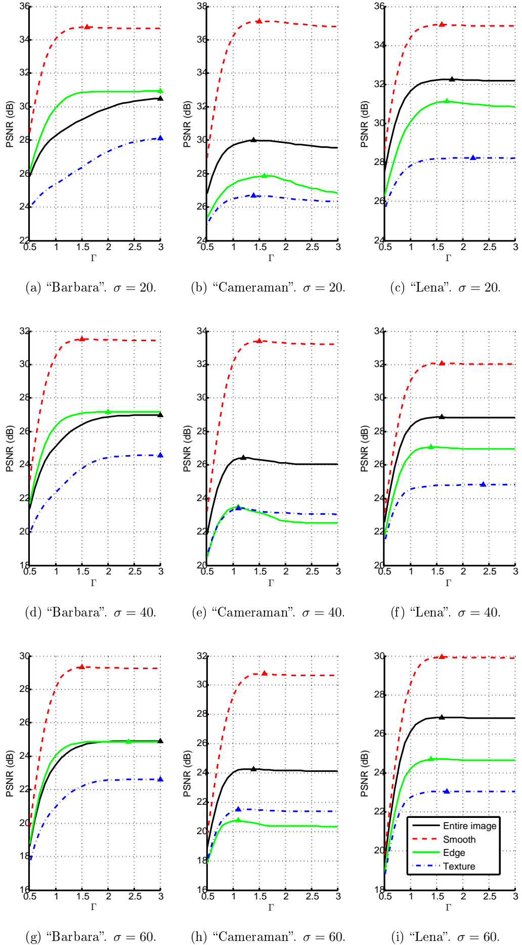
Figure 3.8: Dependence of calculated PSNR on \Gamma for SA-DCT filtering.
