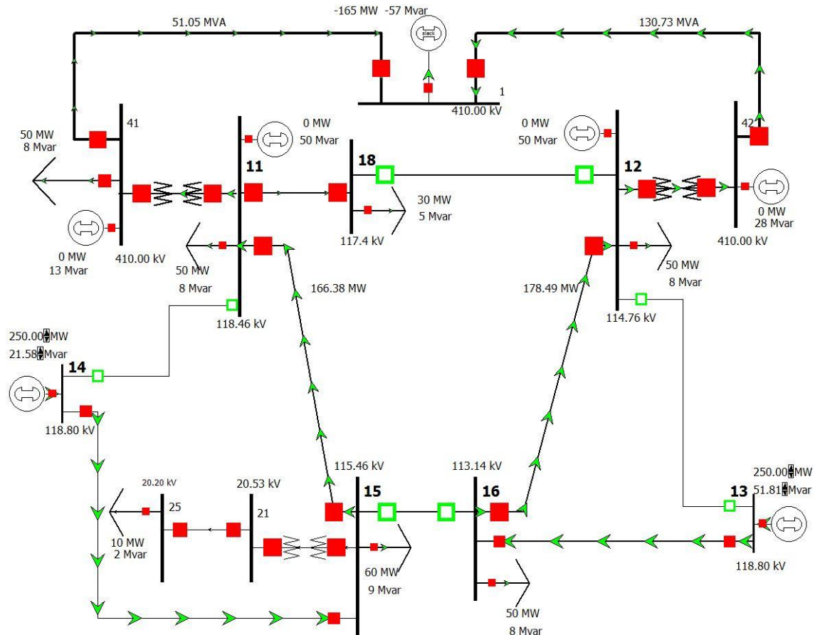
Figure 2.3. The HVDN test system in the maximum load situation and with wind farms connected to the existing 110 kV substations.
