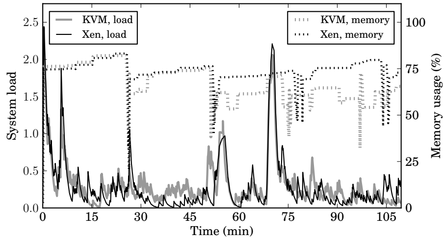
Figure 4.7: A virtual machine’s system load and memory usage during a httperf run.
