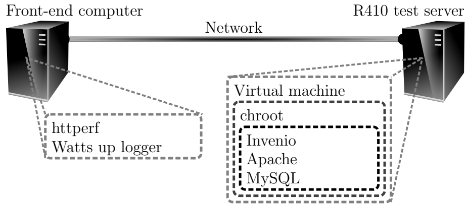
Figure 3.3: The web server test setup. Invenio , Apache and MySQL were running inside a chroot jail inside a virtual machine on the R410. In the front-end computer, HTTP workloads were generated with httperf and Watts up logger was recording the R410's power consumption. Routers in the network are not illustrated.
