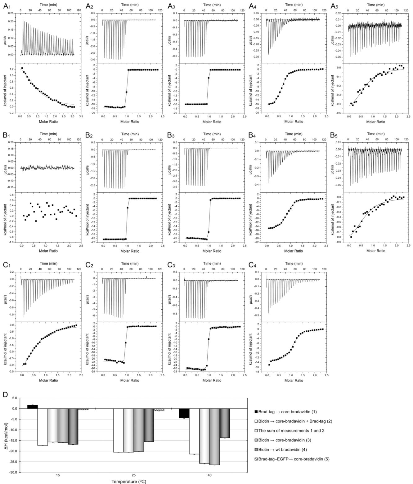
Figure 5. ITC analysis of ligand binding. Thermograms of measurements performed at three different temperatures ( A ) 15°C, ( B ) 25°C and ( C ) 40°C are shown. At each temperature, core-bradavidin was first titrated with Brad-tag (1), followed by competitive titration with biotin (2). As a control measurement, core-bradavidin was titrated with biotin only (3). In order to prove that the intrinsic Brad-tag decreases the affinity towards biotin, wt bradavidin was also titrated with biotin (4). In addition, core-bradavidin was titrated with Brad-tag-EGFP at 15 and 25°C (5). ( D ) Comparison of the binding enthalpies of all measurements at different temperatures. Brad-tag had a clear effect on the binding enthalpy of the competitive titration with biotin at 15°C (endothermic Brad-tag binding) and 40°C (exothermic Brad-tag binding). At 25°C, the enthalpy of competitive titration was equal to that of titration with biotin only (no detectable binding of Brad-tag to core-bradavidin). doi:10.1371/journal.pone.0035962.g005
