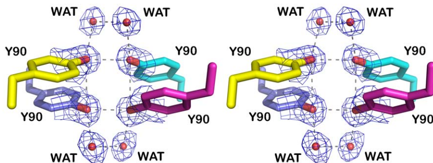
Figure 3. Four tyrosine residues at the intersection of all four subunit interfaces in bradavidin. A stereo view. The tyrosine residues are shown as stick models with different colouring for the different subunits (subunit I, blue; II, cyan; III, magenta; and IV, yellow). Structural water molecules are shown as red spheres. Electron density map (a weighted 2FO-FC map; sigma level 1) around the water molecules and the side chain oxygen atoms of Tyr90 is shown in blue. Putative hydrogen bonds are indicated with grey dashes. doi:10.1371/journal.pone.0035962.g003
