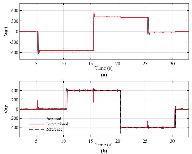
Fig. 6. (a) Active power step change. (b) Reactive power step change
