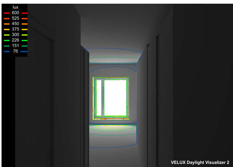
Figure 8 Illustration of illuminance of apartment 1-A during March at 12:00, with overcast sky.
