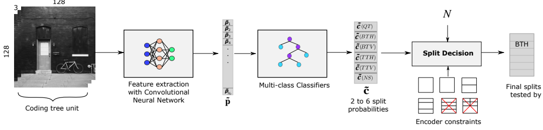
Fig. 1. Workflow diagram of the proposed fast block partitioning scheme for VVC under RA configuration. The current luminance CTU \mathbf{B}_{cur} plus its two CTUs of reference \mathbf{B}_{MV1} and \mathbf{B}_{MV2} which are processed by a CNN to predict \hat{\mathbf{p}} , a vector of N_p probabilities describing all edges at each 4 \times 4 block. The vector \hat{\mathbf{p}} is then processed by the MCC to predict probabilities of the six partitioning options through the vector \hat{\mathbf{c}} . The top- N splits of the highest probabilities are tested by the RD optimization of the encoder to select the optimal split in terms of RD-cost.
