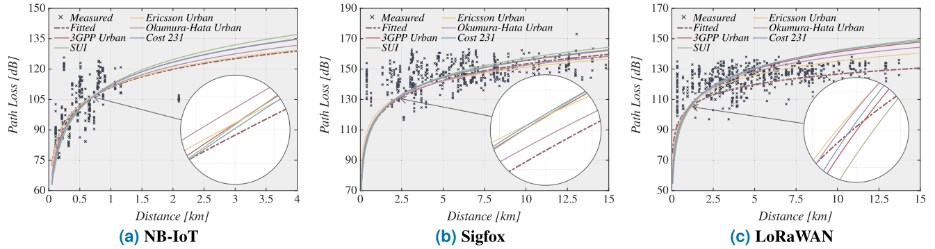
FIGURE 8. Comparison of fitted model derived from Ostrava data and models tuned to Brno data.
