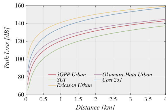
FIGURE 1. Comparison of propagation models.
