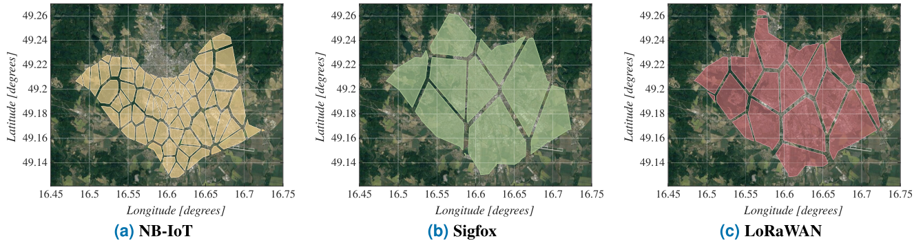
FIGURE 3. Voronoi diagram of LPWAN BSs in the city of Brno.
