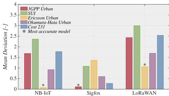
FIGURE 7. Tuned models accuracy in the city of Brno.
