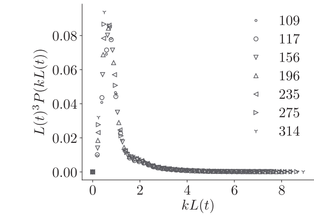
Fig. 8. Scaled Fourier transformed correlation function at different times.
