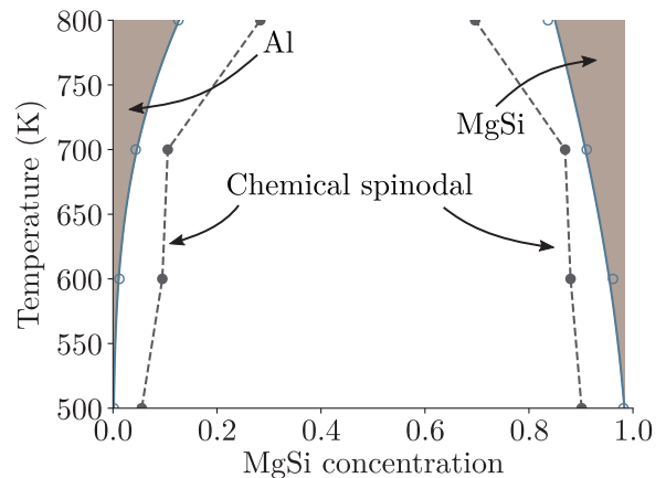
Fig. 4. (a) Free energy curves at four temperatures for the Al 2-2x Mg x Si 3x system. The common tangent and the concentration of the inflection points are shown as examples. (b) Corresponding phase diagram.
