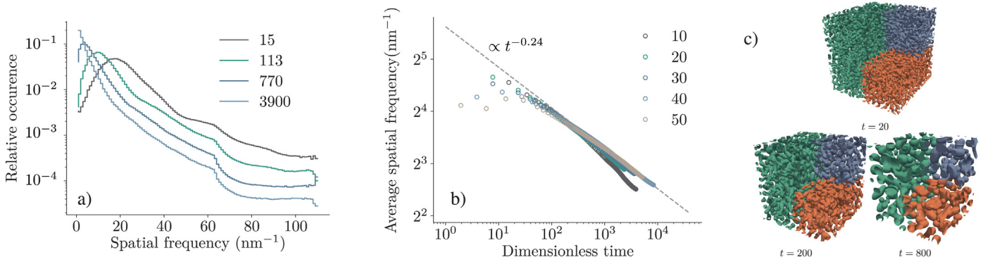
Fig. 7. (a) Radially averaged Fourier transformed concentration field at dimensionless times 15, 113, 770 and 3900. (b) Time evolution of the average spatial frequency at various solute concentrations and (c) Visualisation of the coarsening process. The colors are included for visual clarity. (For interpretation of the references to color in this figure legend, the reader is referred to the web version of this article.)
