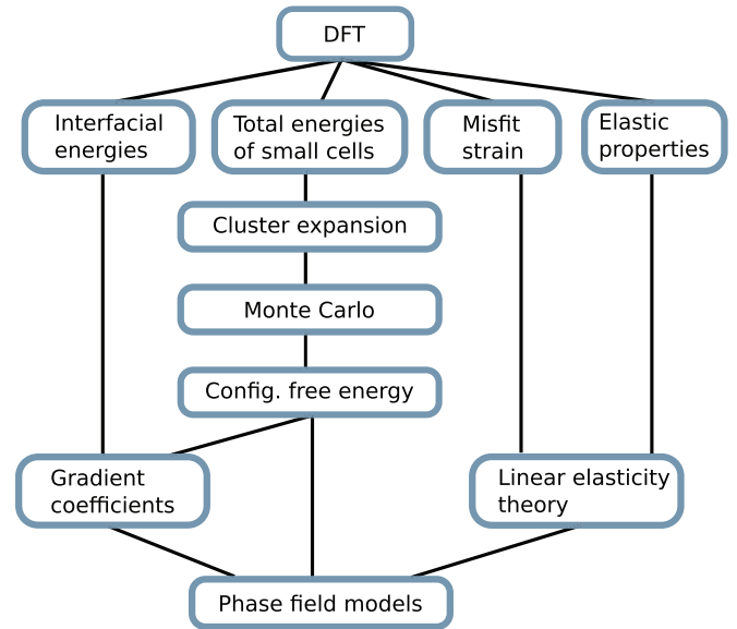
Fig. 2. Hierarchical overview of the methods used to study Al–Mg–Si alloys. The process starts from DFT calculations, and the results are propagated through several layers until the final phase-field model is obtained.
