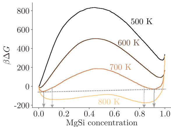
Fig. 4. (a) Free energy curves at four temperatures for the Al 2-2x Mg x Si 3x system. The common tangent and the concentration of the inflection points are shown as examples. (b) Corresponding phase diagram.
