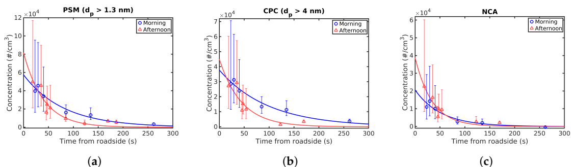
Figure 4. The mean concentrations of particles (a) larger than 1.3 nm (PSM), (b) particles larger than 4 nm (CPC) and (c) NCA for morning and afternoon measurements together with exponential fits to data and with geometric standard deviations. Background concentrations have been subtracted from the data. The fitting parameters used are presented in Table 2.
