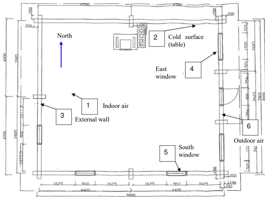
Fig. 2. Location of dataloggers in case building 5.
