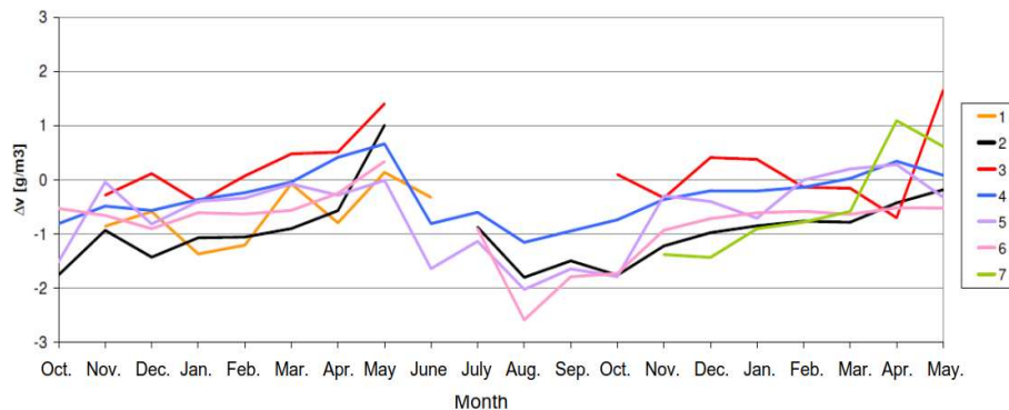
Fig. 4. The monthly average differences between the indoor and outdoor water vapour content of studied case buildings during 2007-2009.
