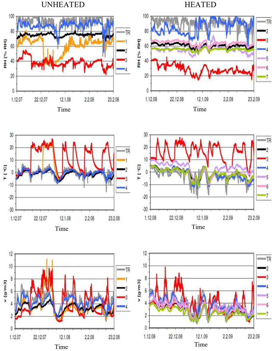
Fig. 3. Daily average indoor and outdoor conditions of unheated case buildings from 1.12.07-23.2.08 are presented in left and constant output heated case buildings from 1.12.08-23.2.09 are presented in right. Upper figures show relative humidities, middle show temperatures and lower show water vapour concentrations.
