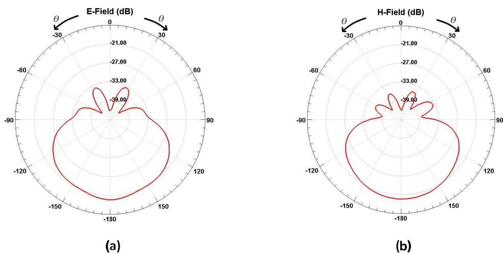
Figure 23. 3-D gain pattern of the far-field antenna at 2.45 GHz [Publication IV].
