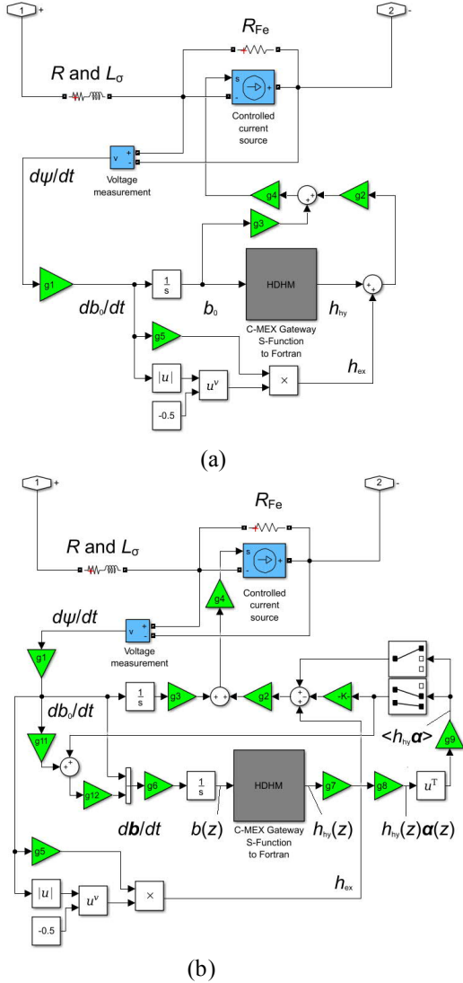
Fig. 6 Illustration of the Simulink implementations of the inductor model (a) without and (b) with skin effect. Notation \langle \cdot \rangle denotes averaging over the lamination thickness z \in [-d/2, d/2] . The gains are explained in Table II. The paths producing h_{ex} result in algebraic loops.
