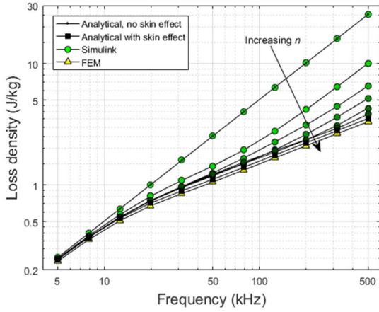
Fig. 9 Validation of the eddy-current loss model implementation in Simulink by comparing simulated energy-loss densities with n = 1, 2, 3, 4, 5, 6 skin-effect terms to (39) with and without X(x) at different frequencies of a sinusoidal average flux density b_0(t) . Finite-element simulation results are also shown.
