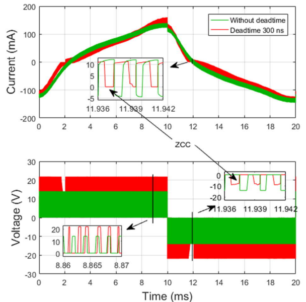
Fig. 13 Simulated primary current and voltage waveforms at 500 kHz switching frequency both without and with deadtime when n = 3 . The insets show the zero-current clamping (ZCC) when the deadtime is accounted for.
