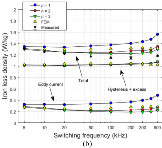
Fig. 11 Simulated iron-loss densities with different switching frequencies and different numbers of skin-effect terms n (a) without deadtime and (b) with deadtime of 300 ns. FE simulation results and measured losses with error in the case of 300 ns deadtime are also shown.
