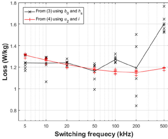
Fig. 2 Losses measured from the test inductor at 5 – 500 kHz switching frequencies. The markers denote the six separate measurements for each switching frequency. The lines are drawn through the average values. Results calculated with (3) and (4) are shown.
