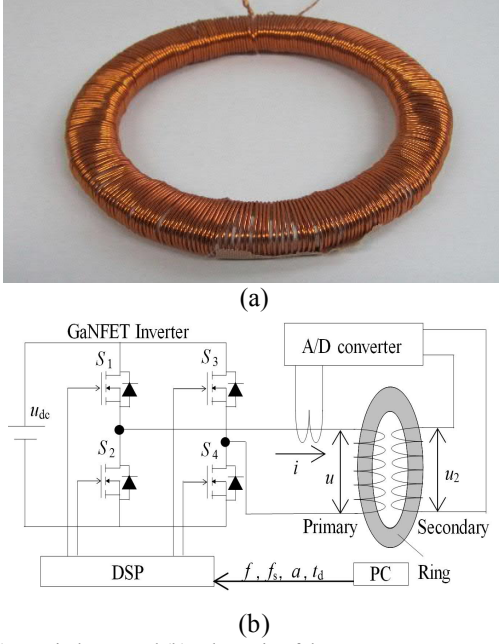
Fig. 1 (a) Test inductor and (b) schematic of the measurement setup.
