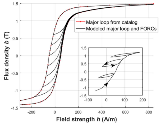
Fig. 4 Major hysteresis loop for Nippon 35H300 electrical steel digitized from the manufacturer catalog as well as the major loop and a set of ascending first-order reversal curves obtained from the history-dependent hysteresis model. The inset shows some simulated minor loops.
