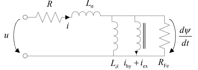
Fig. 5 Equivalent circuit of an inductor with an air gap and an iron core with hysteresis, eddy-current and excess losses.
