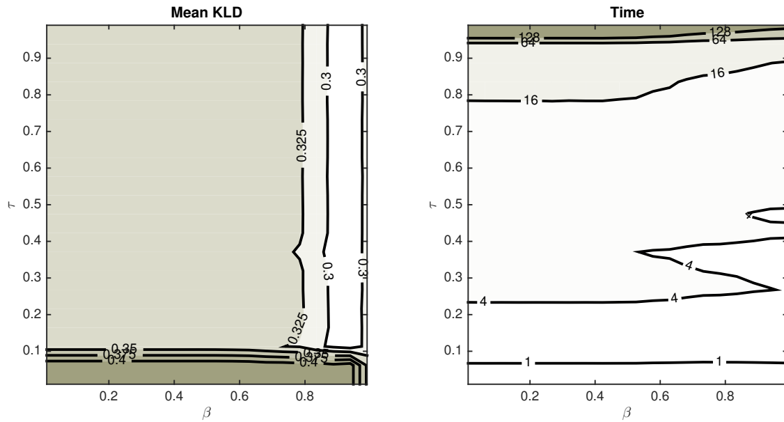
Fig. S-3. Effect of parameters \tau and \beta on the mean KLD and computing time
