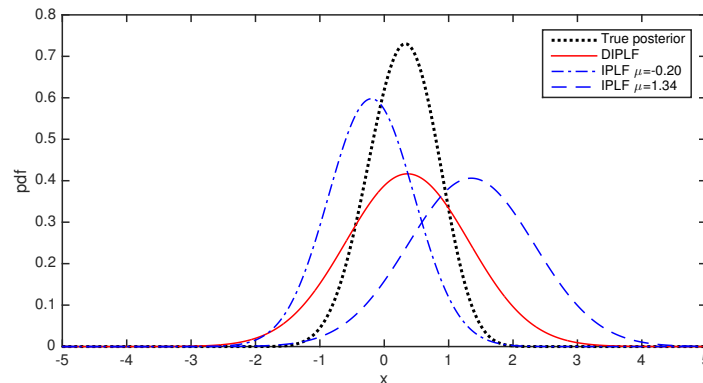
Fig. S-2. True posterior compared to the oscillating estimates of IPLF and the estimate provided by DIPLF
