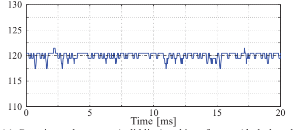
(a) Capacitor voltage v_{C1} (solid line) and its reference (dash-dotted line) in [V].
