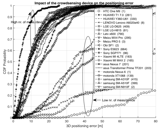
Fig. 9. Impact of the crowdsensing device type and the number of measurements per device on the positioning error.
