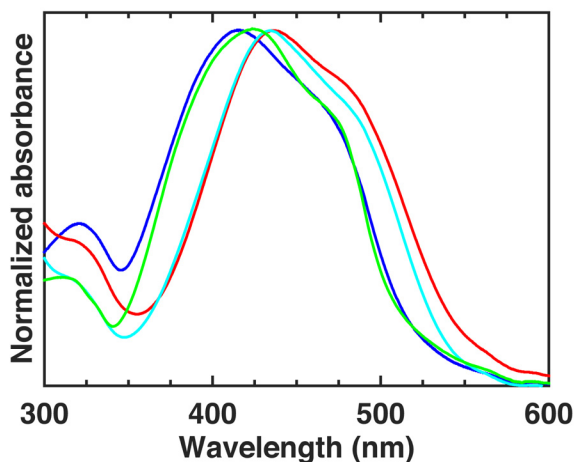
Figure 2. Normalized UV-visible absorption spectra of spin-coated films of p(1) 0.25 (red), p(2) 0.25 (blue), p(3) 0.25 (cyan), and p(4) 0.25 (green).
