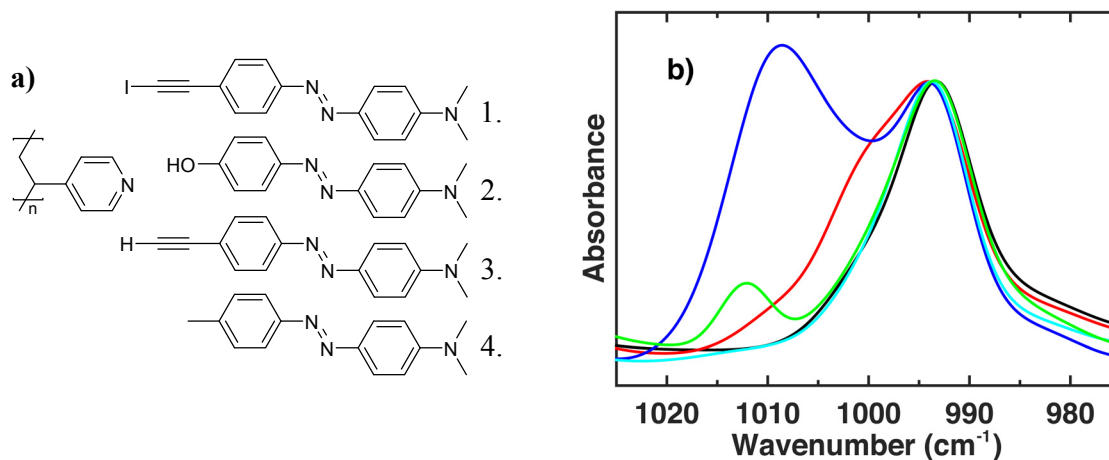
Figure 1. a) Molecular structures of the complexes studied. b) IR spectra of the pyridine stretching vibration in pure spin-coated P4VP (black), p(1) 0.25 (red), p(2) 0.25 (blue), p(3) 0.25 (cyan), and p(4) 0.25 (green).
