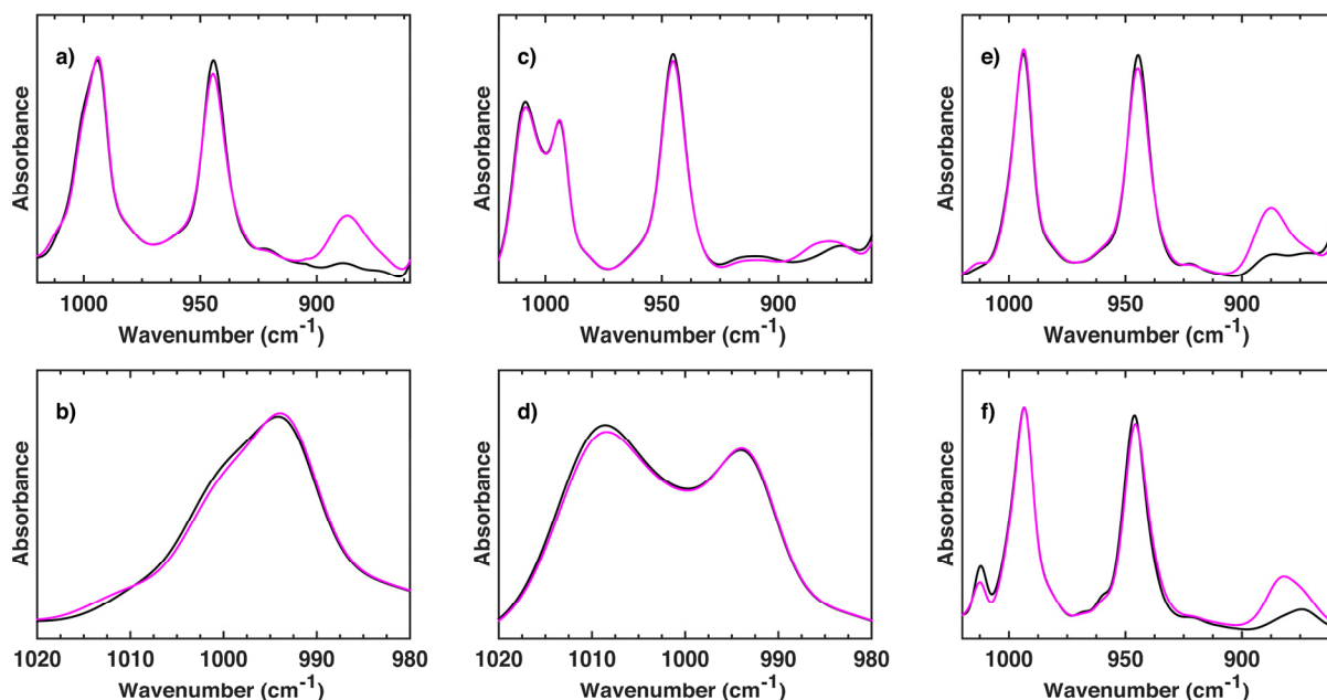
Figure 5. Static IR spectra recorded in the dark (black) and under (pink) illumination of 450 nm unpolarized light for a) and b) p(1) 0.25 , c) and d) p(2) 0.25 , e) p(3) 0.25 , and f) p(4) 0.25 .
