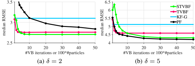
Figure 4. Convergence of the STVBF with q = 10 . Ten STVBF iterations is enough to outperform TVBF. One additional VB iteration gives the same accuracy gain as 100 additional PF particles.
