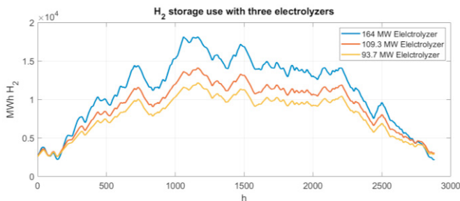
Fig. 3. Hydrogen storage use with three different capacity electrolyzers.
