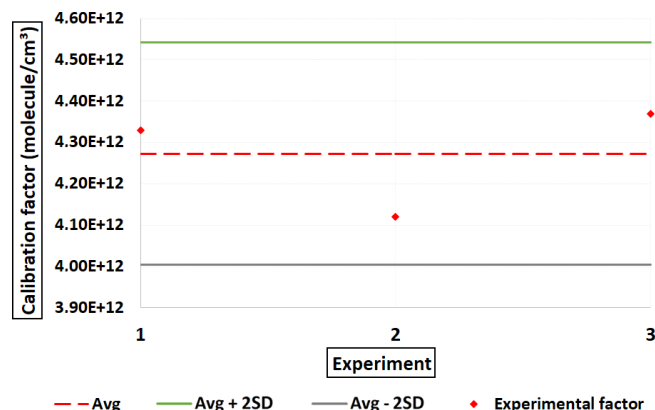
Figure 7. Malonic calibration coefficients obtained within a 95 % confidence interval. The red symbols depict the factors obtained from each experiment performed.
