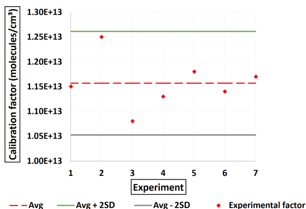
Figure 5. Oxalic acid calibration coefficients obtained showing the mean (red line) and 95 % confidence intervals (green and gray lines). The red symbols depict the calibration factors obtained from each experiment.
