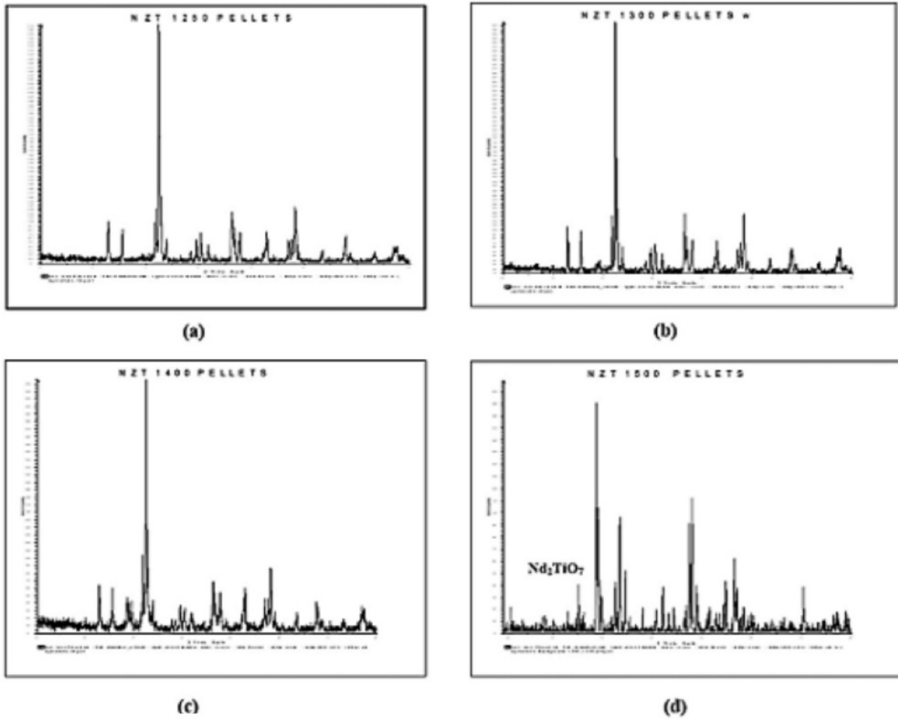
Fig. 8. XRD image of NZT samples in different temperatures.
