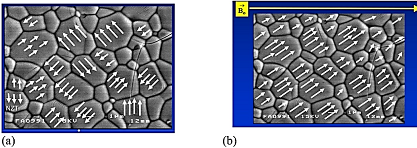
Fig. 10. (Color online) (a) Unmagnetized sample Pellet of NZT sintered at 1400°C and (b) Magnetized pellet of NZT 1400°C in direction of B_0 \rightarrow .
