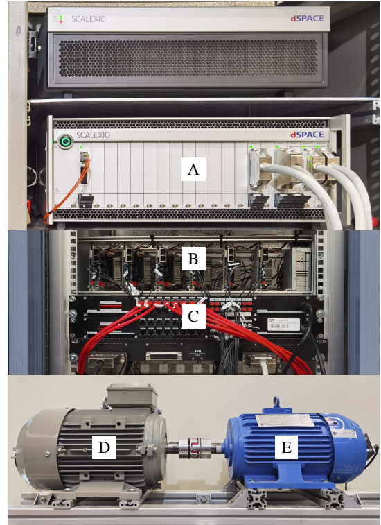
Fig. 4: Setup of the electrical drives test bench. A: dSPACE SCALEXIO real-time control system, B: Back-to-back 3L-NPC converters, C: Interface, D: IM, E: PMSM
