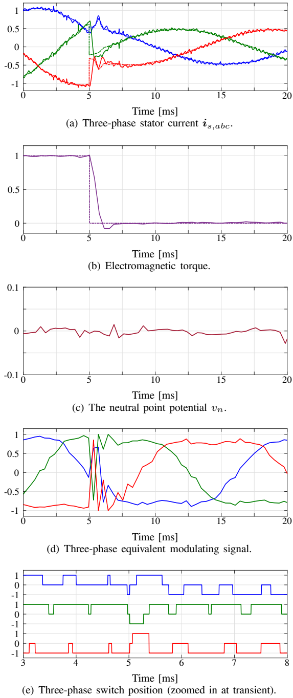
Fig. 10: Experimental results of direct MPC at a torque reference step-down transient.
