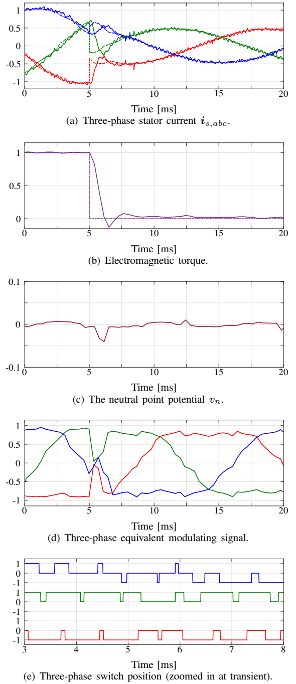
Fig. 11: Experimental results of FOC at a torque reference step-down transient.
