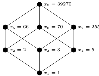
Fig. 2. An example of a GCD closed set with eight elements such that the corresponding LCM matrix is singular.
