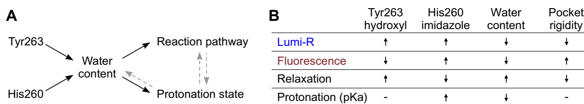
Fig. 6 Summary of the results obtained in the study. A Simplified scheme of the events related to the coordinated water content in the chromophore-binding pocket. H260 and Y263 affect the water network, which then affects the chosen reaction pathway (Lumi-R, fluo-
