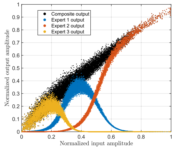
Fig. 5. Illustration of the outputs of the individual experts weighted by their corresponding gating functions and the composite model output. Direct PA modeling experiment with LMBA GaN PA at 2.1 GHz.
