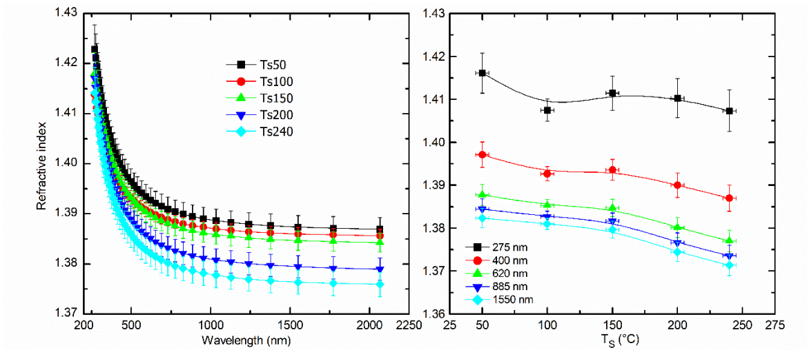
Fig. 1. Dispersion curves of the MgF 2 thin films and refractive index at selected wavelengths as a function of substrate temperature. The uncertainty bars represent 90 % level of confidence.
