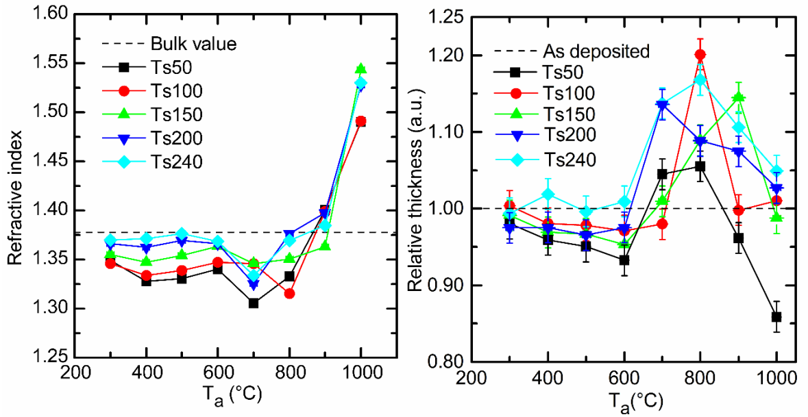
Fig. 5. Refractive indices and film thicknesses measured at \lambda=632.8 nm of the MgF_2 thin films annealed in different temperatures. Bulk value by Heavens et al.[36]. The uncertainty bars represent 90 % level of confidence.
