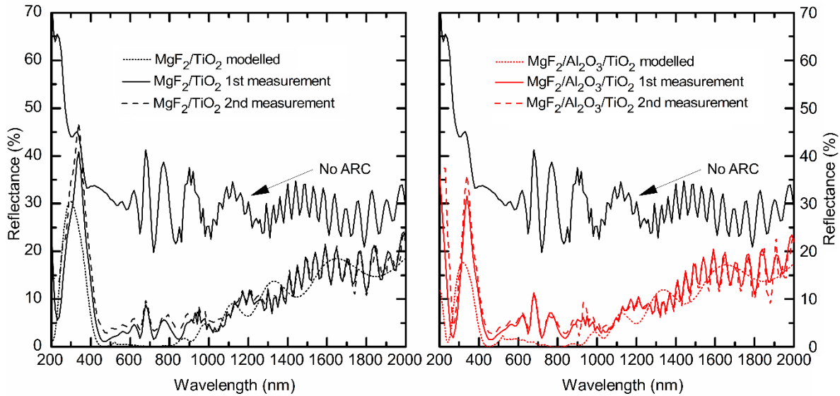
Fig. 8. Reflectance measurements of two different ARCs on a triple-junction solar cell right after deposition (1 st measurement) and after a year exposure to ambient conditions (2 nd measurement) and as a comparison the reflectance for the simulated design of the both ARC structures on top of the solar cell.
