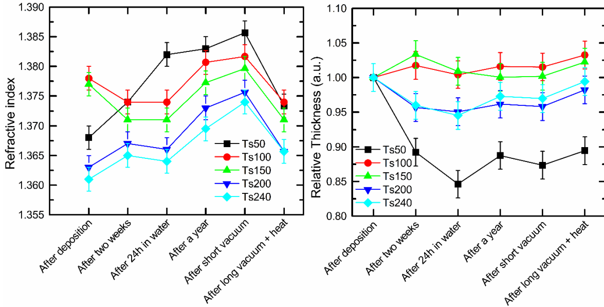
Fig. 3. Refractive indices and film thicknesses measured at \lambda=632.8 nm of the MgF_2 thin films with different post deposition conditions. The uncertainty bars represent 90 % level of confidence.
