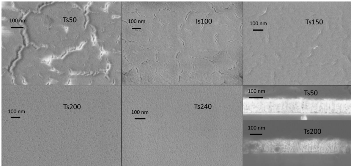
Fig. 4. Sample surfaces of the MgF_2 thin films imaged with SEM after a year exposure to ambient conditions and cross-sectional images of the samples grown in 50 °C and in 200 °C.
