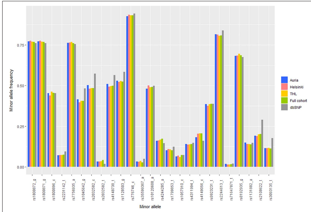
Figure 2. Minor allele frequencies for the three sub-cohorts (Auria Biobank, Helsinki Biobank and THL Biobank), the combined full cohort and earlier reported data for the European population (dbSNP).
