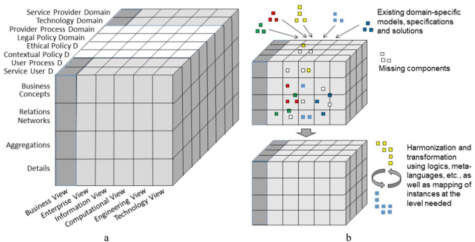
Figure 1. AIS representation, design and implementation enabling advanced interoperability and integration acc. to ISO 23903
