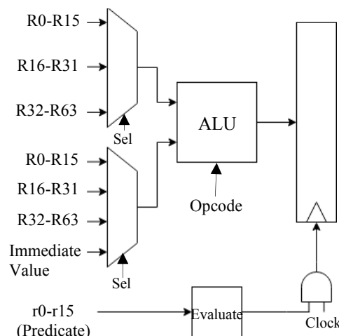
Fig. 3. Inputs to the ALU
