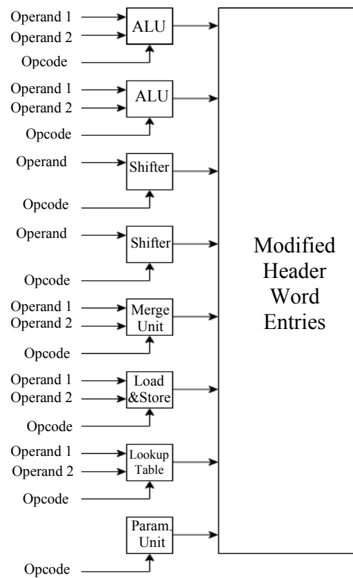
Fig. 2. A Group of Functional Units (GFU)
