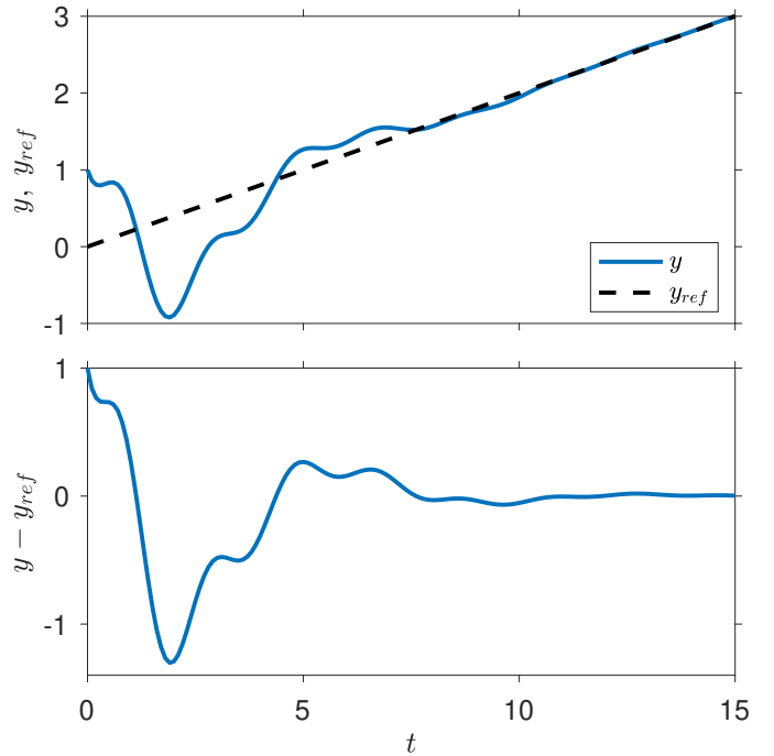
Fig. 1. Above: the reference signal y_{ref} and the output y . Below: the regulation error e = y - y_{ref} .
