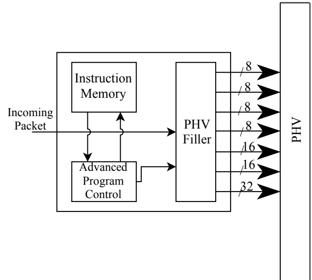
Fig. 5. High-level view of the packet parser
