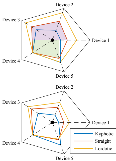
Fig. 3. Inclination angles for two of the subjects. There are five data points on each curve that represent the inclination angles measured from each device. Each curve represents one of the examined postures.
