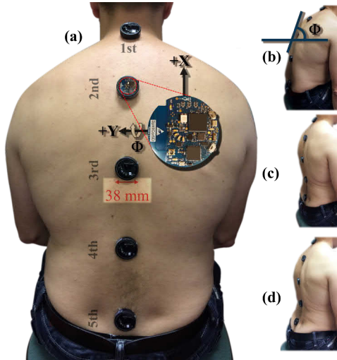
Fig. 1. The placement of the sensors and the axes of acceleration sensitivity (a). Kyphotic (b), straight (c) and lordotic (d) postures emulated by subject number 3. The angle of interest is indicated by \phi (b).
