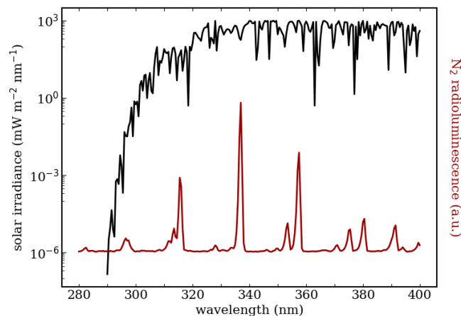
Fig. 1. The spectrum of the sunlight reaching the earth's surface (black) contrasted with the radioluminescence of N_2 (red) in the wavelength range 280 nm to 400 nm. The solar irradiance (AM1.5 Global tilt [4]) is displayed on a logarithmic scale, while the N_2 emissions are shown on a linear scale. For wavelengths longer than 300 nm the spectra overlap. For wavelengths shorter than 300 nm the solar irradiance starkly declines.
