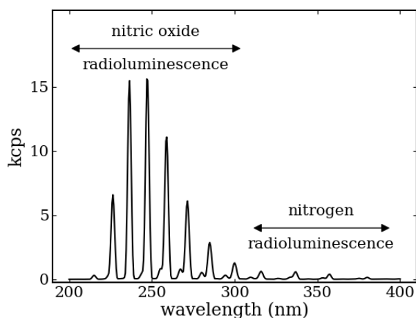
Fig. 2. Radioluminescence spectrum from 200 nm to 400 nm under a constant flow of 18 ppm of NO diluted in N_2 . The NO \gamma -band emissions make up most of the detected light. Almost all of the NO emission lines are in the solar blind spectral region.
