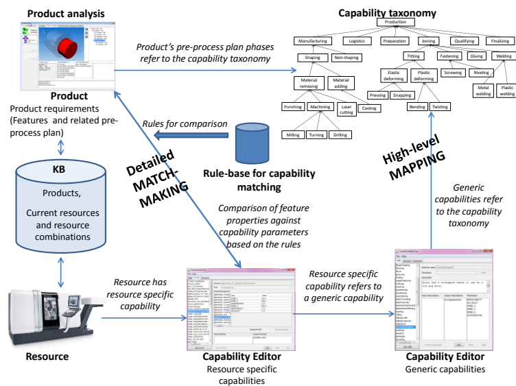
Fig 1.1 Capability-matching framework [2].
