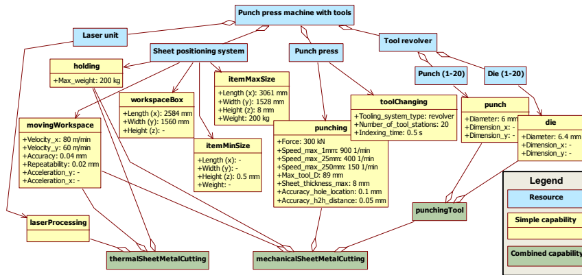
Fig 1.2 Capabilities of the existing punch press machine (Finn-Power LP6 – Series 10).
