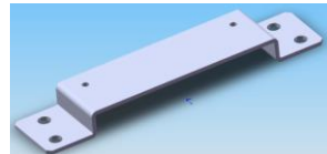
Fig 1.3 The case product. Part’s size is 30,0x158,6 mm. Material thickness is 2,0 mm. Material is galvanized steel. Attributes related to the geometry are presented in the table.
