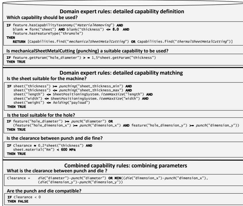
Fig 1.4 Example of the rules used for capability matching in sheet metal manufacturing written in pseudo code.
