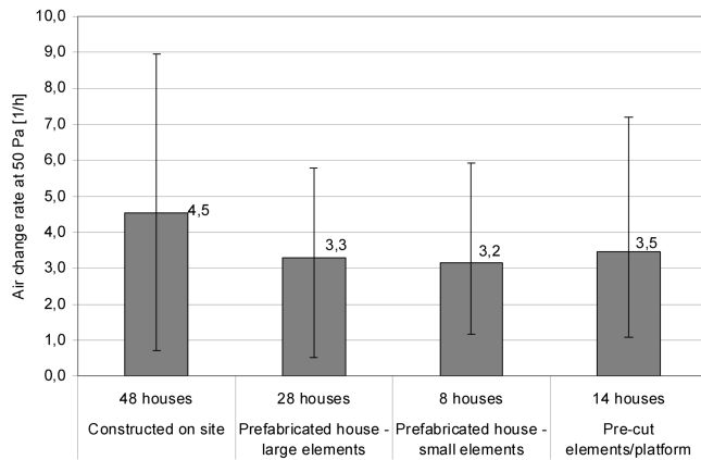
Figure 5 Air change rate at 50 Pa (0.201 in. of water) (1/h) grouped by construction type (average result and the range of results).
