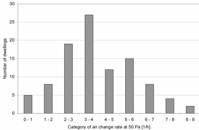
Figure 1 Distribution of air change rates at 50 Pa (0.201 in. of water) (1/h).
