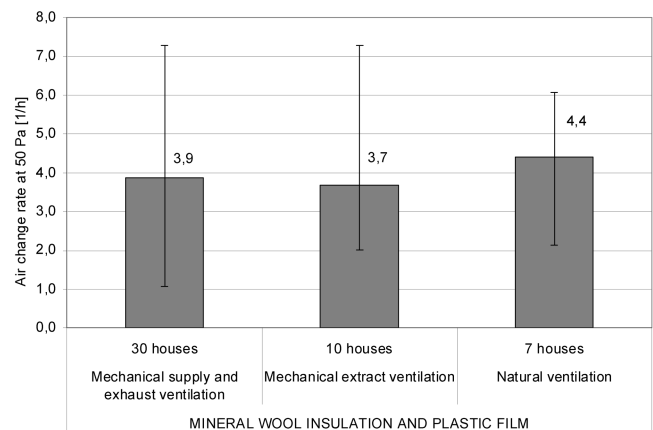
Figure 7 Air change rate at 50 Pa (0.201 in. of water) (1/h) in houses with mineral wool and plastic film grouped by construction type (average result and the range of results).
