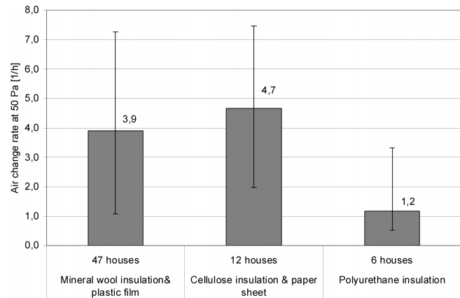
Figure 4 Air change rate at 50 Pa (0.201 in. of water) (1/h) grouped by combinations of insulation and air barrier materials (average result and the range of results).
