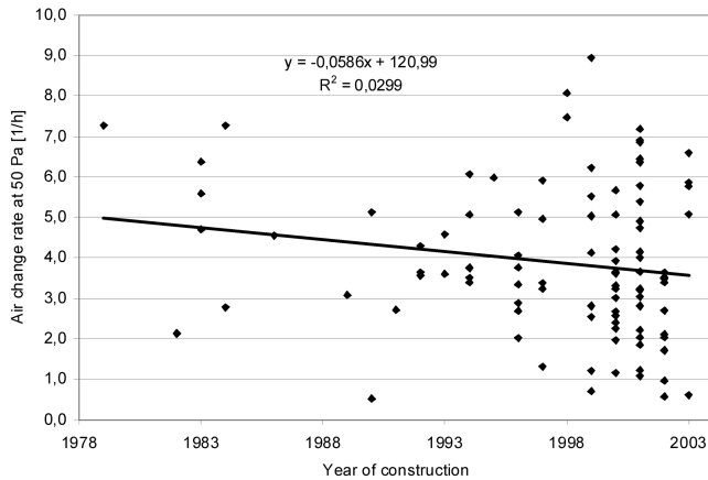
Figure 2 Air change rate at 50 Pa (0.201 in. of water) (1/h) versus the year of construction.
