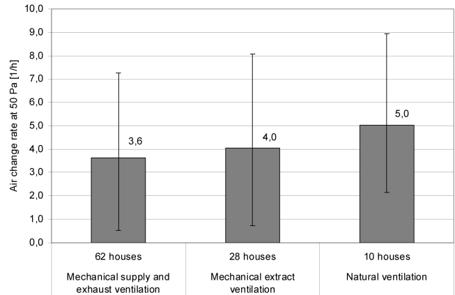
Figure 3 Air change rate at 50 Pa (0.201 in. of water) (1/h) grouped by ventilation system (average result and the range of results).
