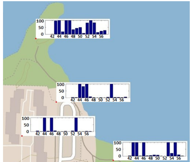
Fig. 2. Illustration of spectrum sensing results of DVB-T measurements in Otaniemi area, Espoo, Finland. Broadcast transmitters use channels 44, 45, 46, and 53. Some of the channels are falsely detected as occupied due to the nonlinear distortion caused by the spectrum-sensing receiver itself, especially in the northern coast area where the broadcast signals are strong.
