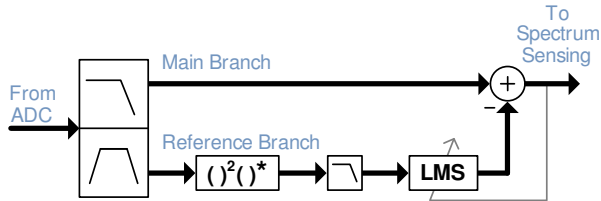
Fig. 3. Block diagram for digital compensation of third-order RF nonlinearity.
