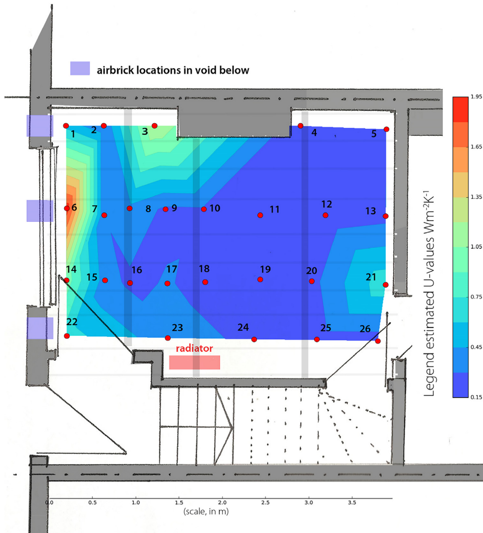
Fig. 9. Linearly interpolated U_p -values as a heat map between observed point U -value locations for the woodfibre insulated floor with the same scale used for the colour legend as in Figs. 7 and 8. An overall significantly reduced heat loss is observed post-insulation, though as expected not as much as the bead-insulated floor. There is still a significant perimeter effect and also a large spread of U_p -values across the floor.
