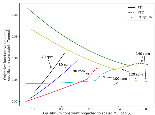
Fig. 10 Projected objective function values for different propeller speeds at time 0.5–1.0 h
