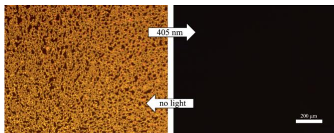
Fig. 4. Photoinduced, reversible smectic-to-isotropic phase transition for St-8•B-6 at 90 °C. Micrographs are taken under POM with crossed polarizers.
