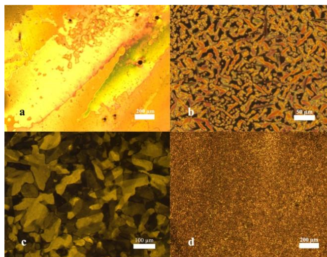
Fig. 4. Representative POM images of the relevant phases observed: a) nematic ( B-6•St-1 at 68 °C), b) smectic A ( B-6•St-8 at 111 °C), c) smectic E ( B-6•St-12 at 50 °C), and d) crystalline ( B-6•St-8 at 25 °C).
