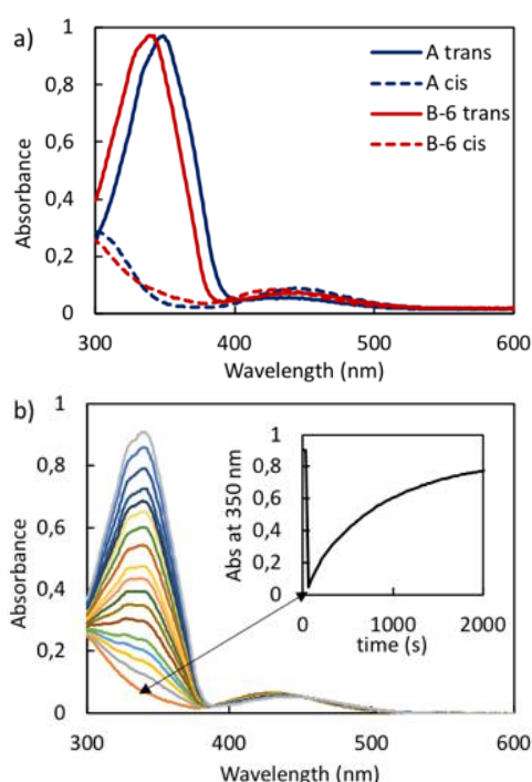
Fig. 2 a) Normalized absorption spectra of A and B-6 in relaxed ( trans ) and photostationary ( cis ) states in toluene at 25 °C, and b) thermal relaxation of B-6 in toluene from photostationary state (inset) to trans , indicated by the increasing absorption at the \pi – \pi^* band.
