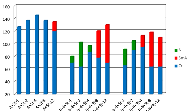
Fig. 3. Chart summarizing the thermal behavior of A and B-n complexes with the stilbazoles St-n . The transitions are reported upon cooling (5 °C/min) for A•St-n and upon heating (5 °C/min) for B-n•St-n .
