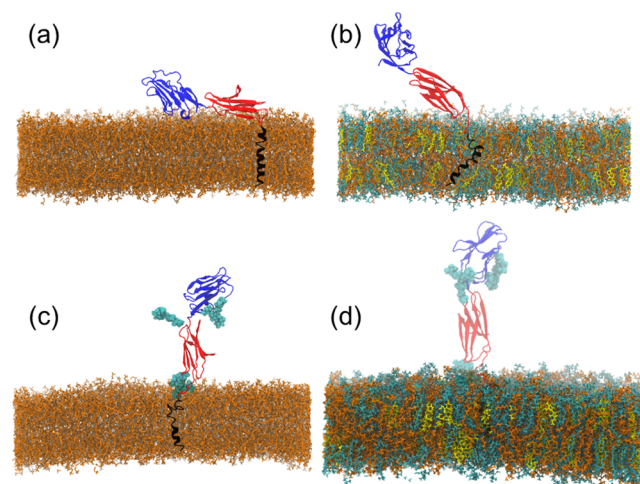
Figure 1. Simulation snapshots of the equilibrium configurations of nonglycosylated CD2 in (a) Ld (Ld-NG) and (b) Lo (Lo-NG) bilayers and of glycosylated CD2 in (c) Ld (Ld-G) and (d) Lo (Lo-G) bilayers. Color code: DOPC (orange), SM (cyan), Chol (yellow), CD2 domain 1 (dark blue), CD2 domain 2 (red), CD2 transmembrane helix (black), and lipid carbohydrate chains (light blue). The glycans attached to CD2 in panels (c) and (d) (Ld-G, Lo-G) are shown in light blue. For clarity, water and ions are not shown.
