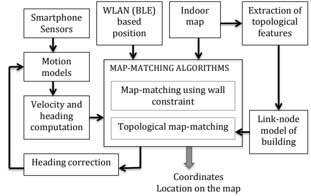
Fig. 9. Approaches to map-matching indoors.
