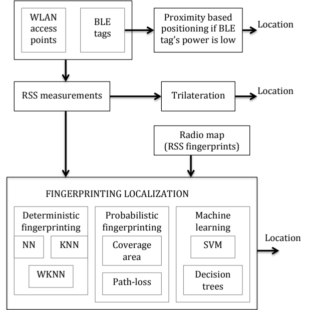
Fig. 2. Approaches for RSS based positioning.
