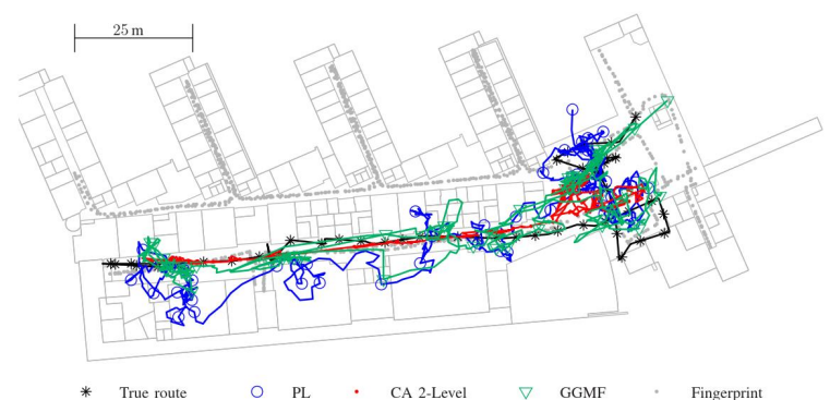
Fig. 8. Field test results for three commonly used WLAN based positioning algorithms. (Reprinted from [7])
