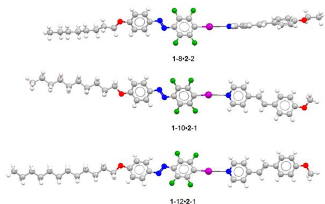
Figure 3. Ball-and-stick representation of the halogen-bonded co-crystals 1-8-2-2, 1-10-2-1, and 1-12-2-1. Strong and directional I \cdots N halogen bonds drive the formation of the supramolecular calamitic structures. Color code: gray, C; white, H; red, O; blue, N; green, F; and magenta, I. Halogen bonds are represented by black dotted lines.
