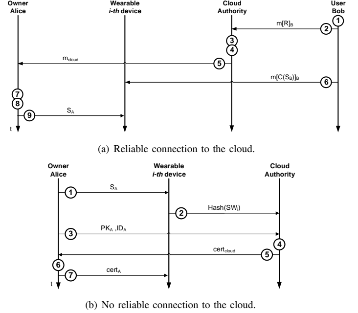
Fig. 6. Wearable device reclaiming protocol.
