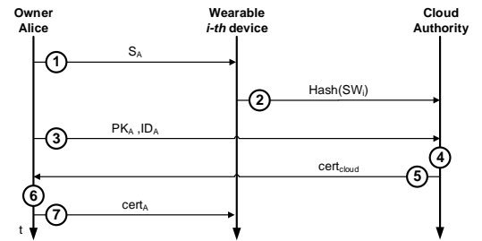
Fig. 4. Wearable device association protocol: connection to the cloud is required.
