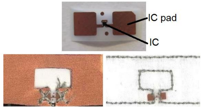
Fig. 3. The used IC strap (up), embroidered cross attachment on copper electro-textile antenna (bottom, left), and antenna embroidered over the IC pads (bottom, right).
