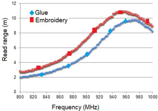
Fig. 4. The attainable read ranges of the copper electro-textile tags with glued and embroidered ICs.
