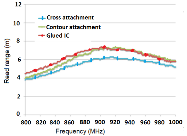
Fig. 6. The attainable read ranges of the embroidered contour tags with different types of IC attachments.
