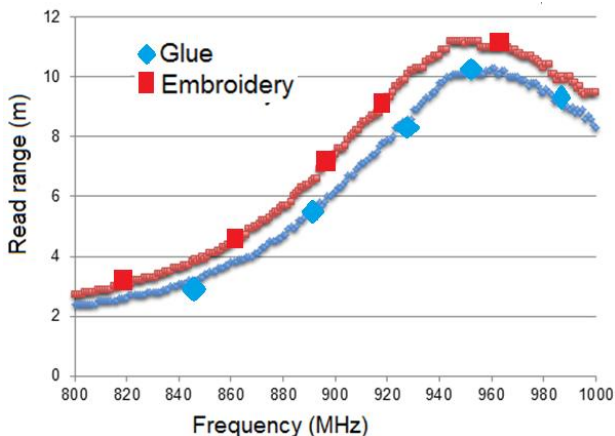
Fig. 5. The attainable read ranges of the nickel/copper electro-textile tags with glued and embroidered ICs.
