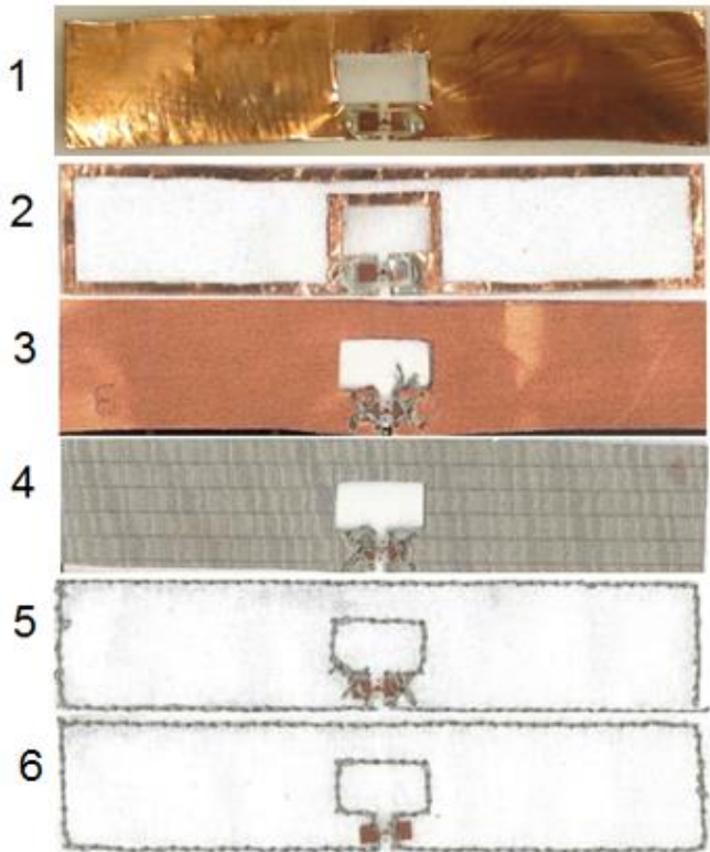
Fig. 2. The ready-made RFID tags: 1. Fully fabricated copper tape tag with a glued IC, 2. Copper tape contour (1 mm) tag with a glued IC, 3. Copper electro-textile tag with an embroidered IC, 4. Nickel/copper electro-textile tag with an embroidered IC, 5. Embroidered contour tag with an embroidered IC, and 6. Embroidered contour tag with IC embroidered together with the antenna.
