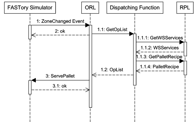
Fig. 4. Sequence diagram for the dispatching scenario
