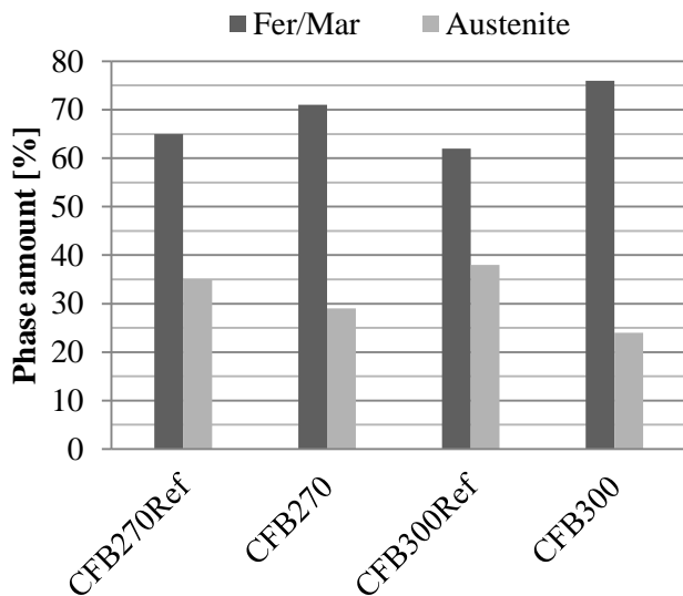
Figure 7. Austenite and ferrite/martensite amounts before (Ref-values) and after erosion tests.
