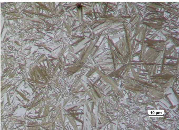
Figure 4: Microstructure of Nital etched CFB300 showing carbide free bainite lath structure enclosing small white areas of austenite and/or martensite (MA).
