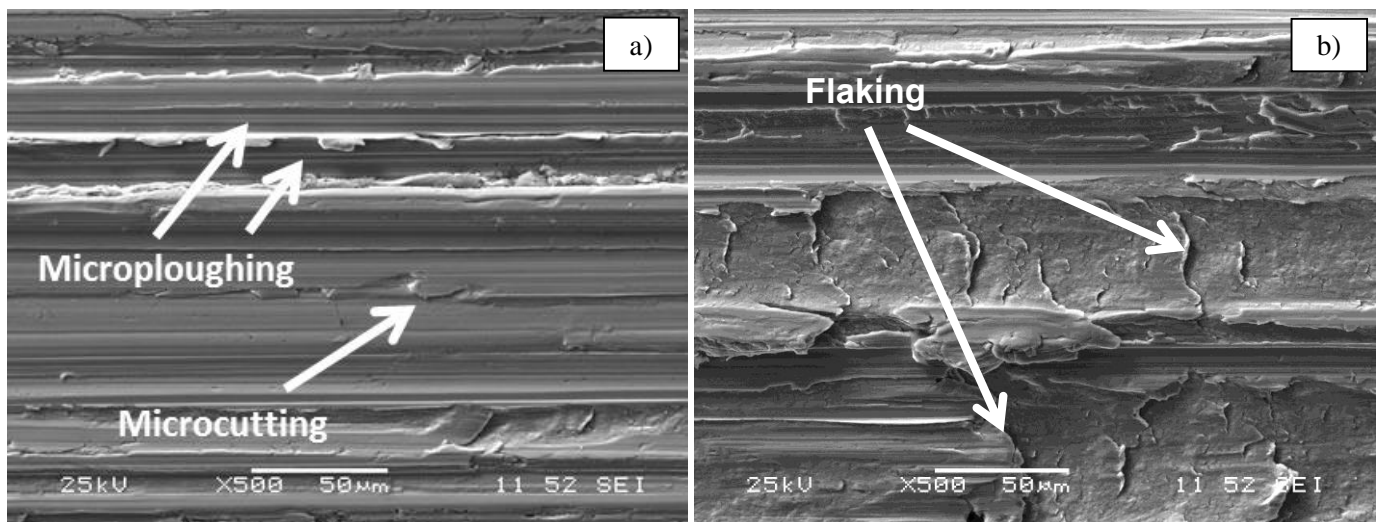
Figure 5: SEM image after abrasion wear test of a) CFB270 showing microcutting, and microploughing, b) QT showing flaking.
