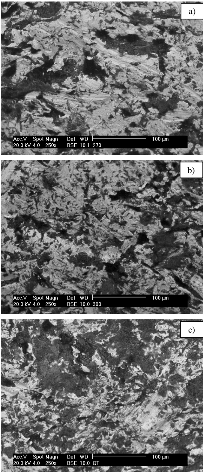
Figure 6: Scanning electron image of erosion tested a) CFB270 sample, b) CFB300 sample and c) QT sample, showing embedded abrasives and short scratches on the erosion surfaces.
