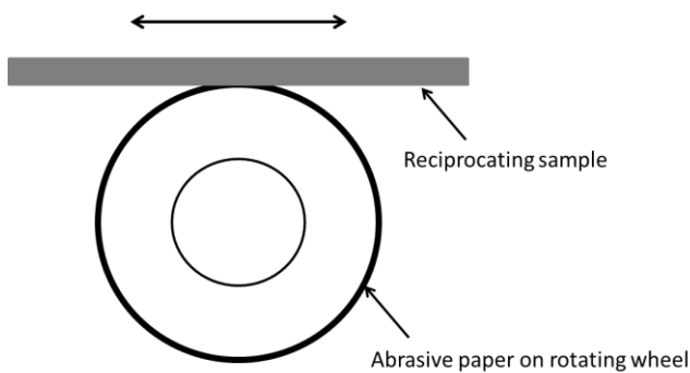
Figure 1: Test configuration for abrasion wear tests.
