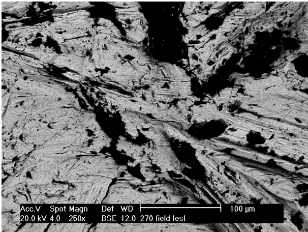
Figure 8. Scanning electron image of field tested CFB270 sample, showing embedded abrasives (dark) and longer scratches on the wear surface.
