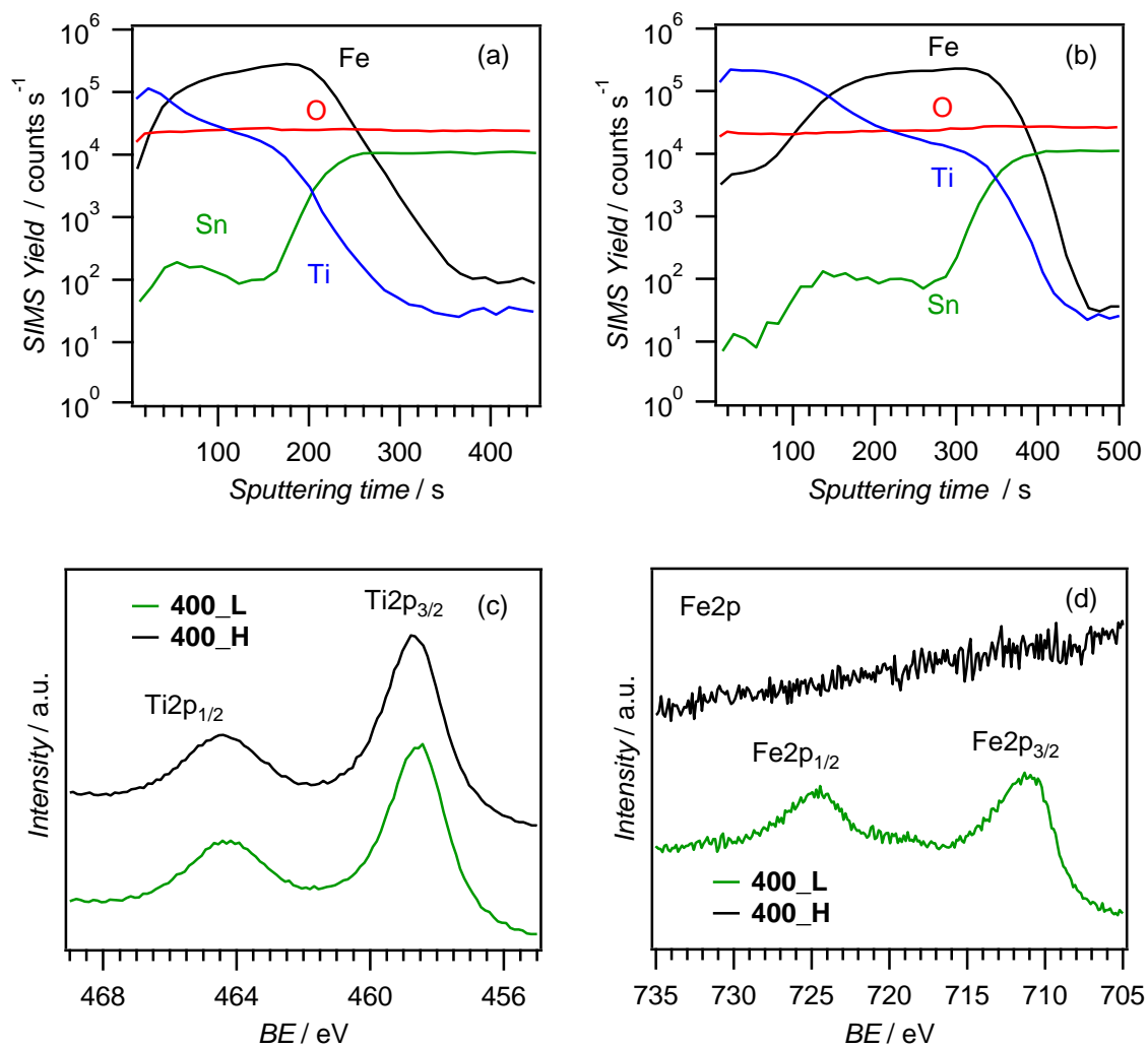
Figure 2. SIMS depth profiles for Fe 2 O 3 -TiO 2 deposits on FTO: (a) 400_L; (b) 400_H. (c) Ti2p, and (d) Fe2p XPS surface spectra for the same specimens.
