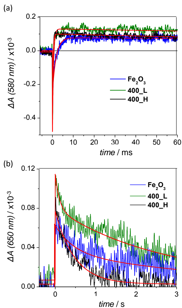
Figure 5. TAS decays for bare \text{Fe}_2\text{O}_3 and \text{Fe}_2\text{O}_3\text{-TiO}_2 samples on a millisecond (a) and a second (b) timescale. Red lines represent exponential fits of raw data.
