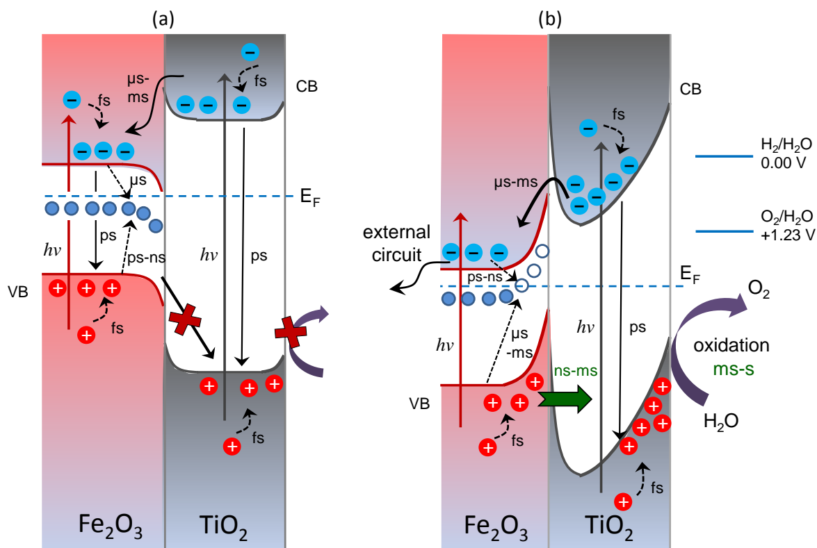
Scheme 1. Schematic energy level diagrams illustrating the photo-activated charge transfer processes and related timescales: (a) without, and (b) with the application of a positive external bias to \text{Fe}_2\text{O}_3 - \text{TiO}_2 photoanodes. The intra-band electron trap states, located a few 100 mV below the conduction band edge of hematite , are also shown. (CB: conduction band, VB: valence band, E_F : Fermi level, fs: femtosecond, ps: picosecond, ns: nanosecond, \mu s: microsecond, ms: millisecond)
